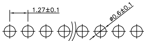
RECOMMENDED P.B.C LAYOUT
